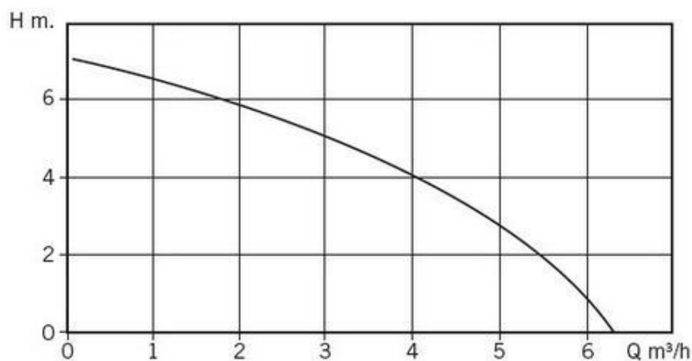
Performance Curve
