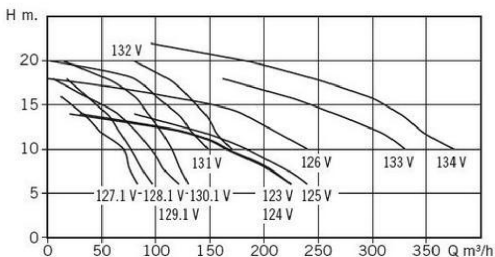
Performance Curve
